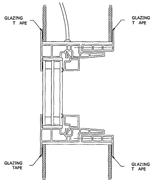
CROSS SECTION DIAGRAM INTERNAL POWER CORD EXIT
